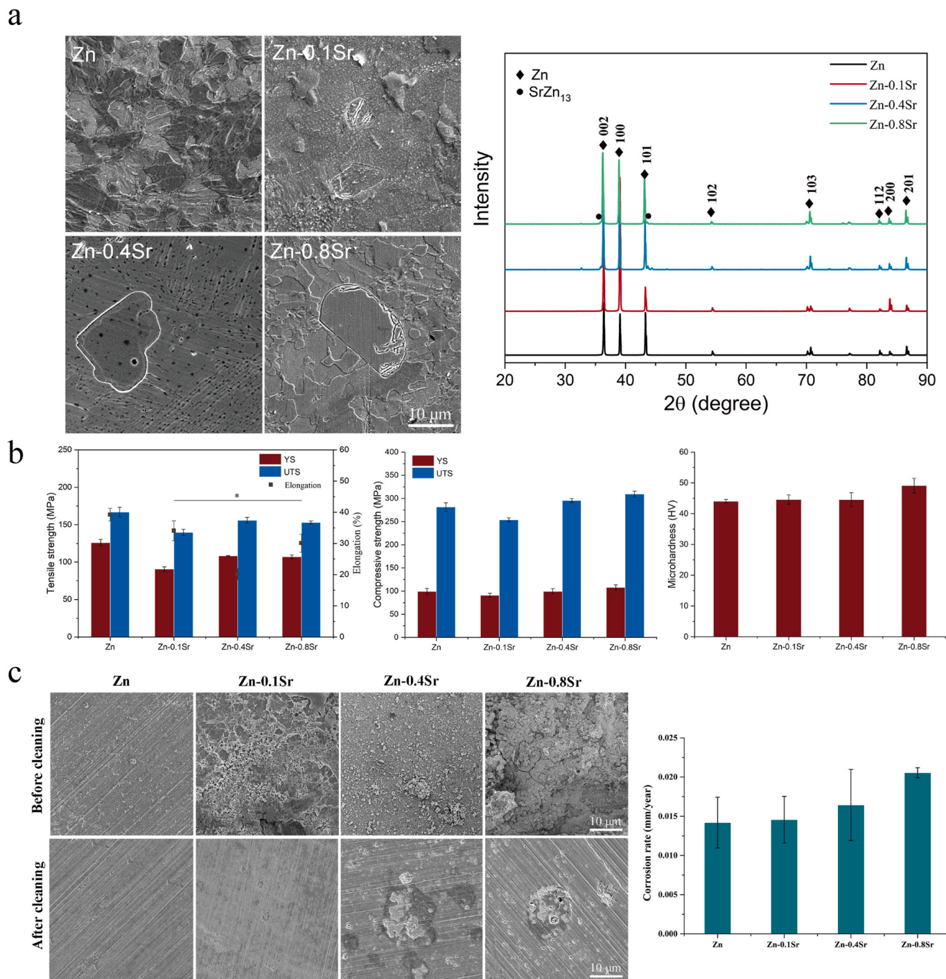
Fig. 1. Material characterization of Zn–Sr alloys. (a) Microstructure and intermetallic phase of pure Zn and the Zn–Sr alloys. (b) Mechanical properties of pure Zn and the as-extruded Zn–Sr alloys. (c) Corrosion morphology after immersion in SBF solution for 30 days.
