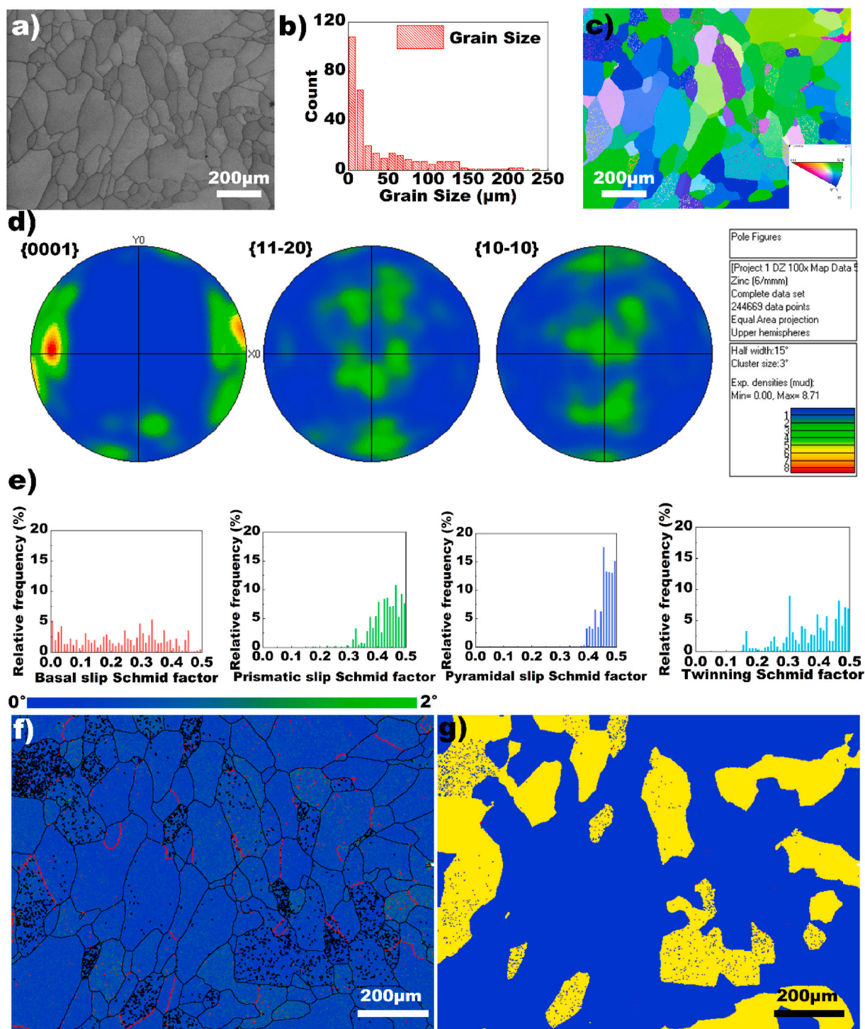
Fig. 3. EBSD measurements of pure Zn after extrusion: a) band contrast map; b) grain size distribution; c) inverse pole figure (IPF) map of Z direction which is parallel to extrusion direction; d) {0001}, {11-20} and {10-10} pole figures; e) Schmid factor distribution of basal slip, prismatic slip, pyramidal \langle a \rangle slip and {10-12} \langle 10-1-1 \rangle deformation twinning; f) Kernel Average Misorientation (KAM) map with color bar corresponding to local misorientation from 0° to 2°; g) recrystallization analysis map where blue represents fully recrystallized region, yellow represents substructure and red represents deformed region.
