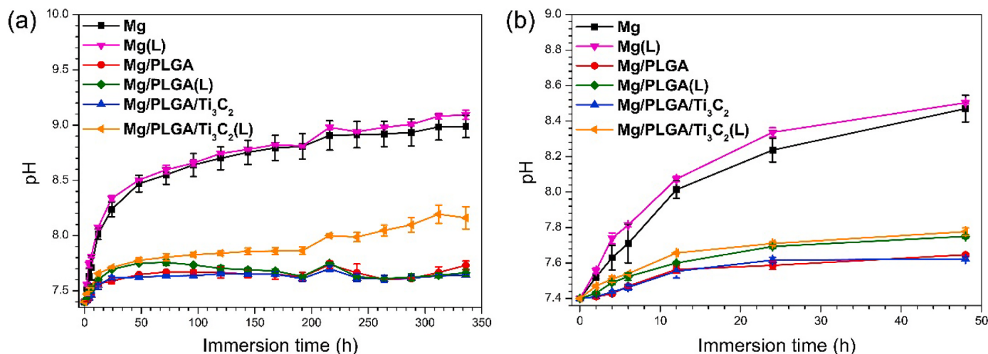
Fig. 7. The pH values evolution of the immersion medium over a period of 14 days.
