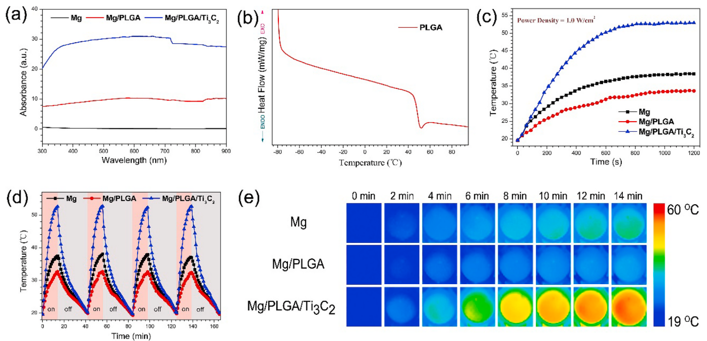
Fig. 3. Photothermal properties measurements under NIR 808 nm laser irradiation: (a) UV-vis-NIR absorption spectra of the different modified samples; (b) Differential scanning calorimetry (DSC) analysis of PLGA; (c) Photothermal heating curves of Mg, Mg/PLGA and Mg/PLGA/Ti 3 C 2 (1.0 W/cm 2 , 20 min); (d) Temperature variations of the different modified samples for 4 cycles; (e) Real-time infrared thermal images of different samples immersed into SBF under continuous 808 nm laser irradiation for 14 min.
