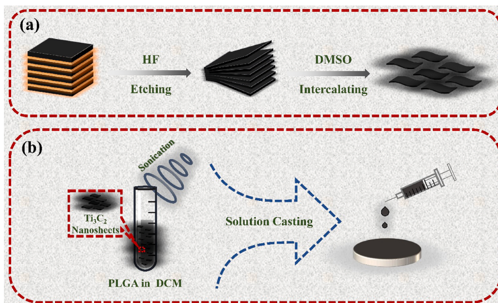
Scheme 1. Schematic diagram of the preparation process of Ti 3 C 2 nanosheets and PLGA/Ti 3 C 2 hybrid coating.
