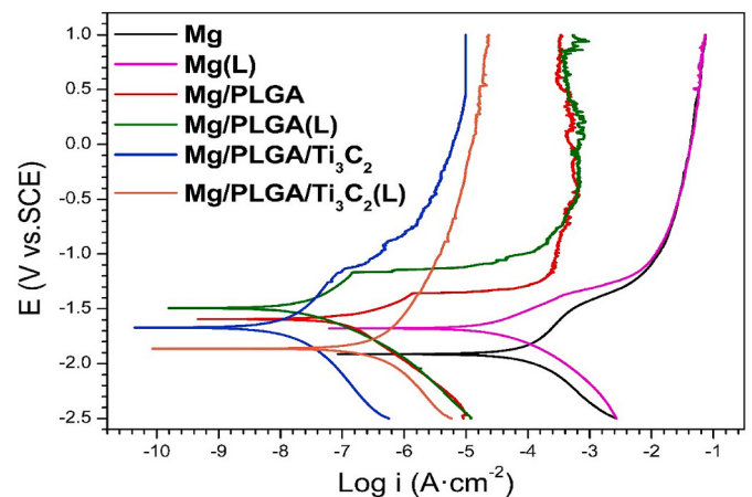
Fig. 4. Potentiodynamic polarization measurements results of each group.
