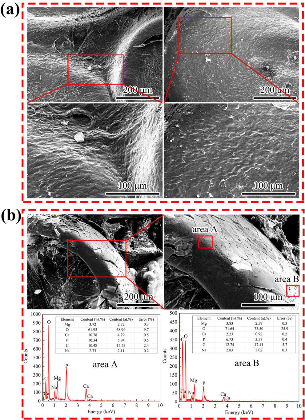
Fig. 8. (a) The status of endothelial coverage on Mg-8.5Li alloy stent after 1 month in iliac artery of minipigs characterized by SEM (typical areas on the strut and in the intermediate spaces of the struts were displayed, tiny particles were salt deposits derived from the tissue fixation and dehydration process.), (b) typical in-vivo corrosion morphology of the stent and corresponding EDS analysis at regions of interest.
