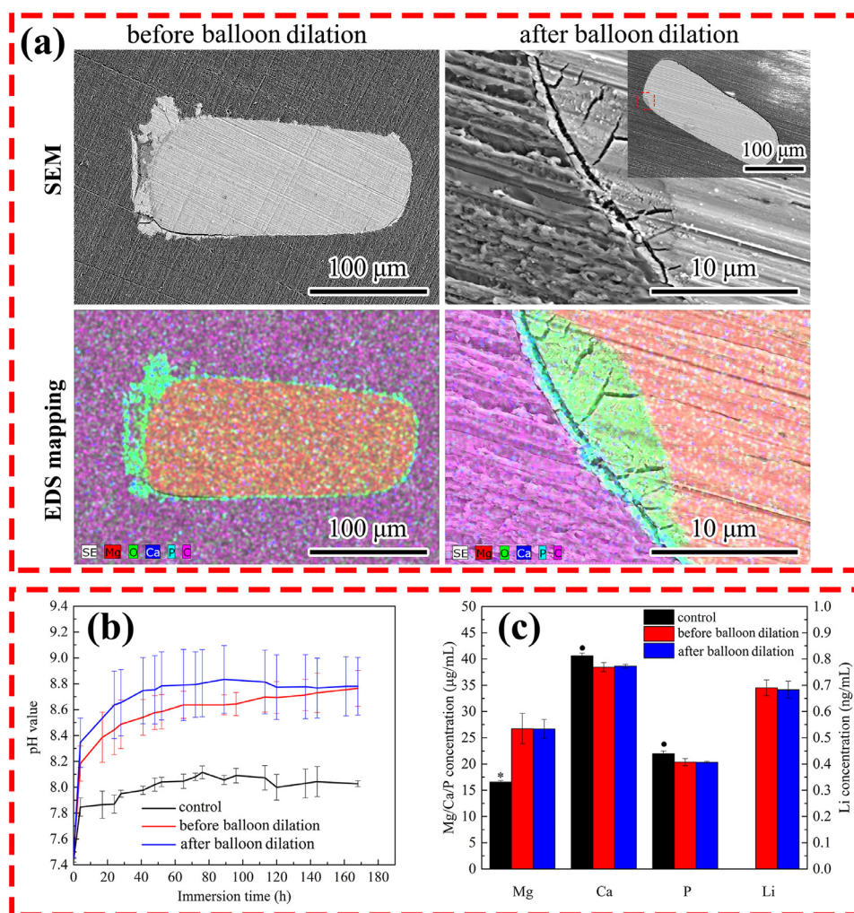
Fig. 5. (a) Cross-sectional morphologies of the degraded stents and corresponding EDS element mapping (red: Mg, green: O, blue: Ca, cyan: P, purple: C), (b) pH variation during a 7-day immersion in Hank's solution at 37 °C, (c) element concentrations (Mg, Li, Ca, P) in Hank's solution after immersion for 7 days, normal Hank's solution as control, * p < 0.05 , * p < 0.01 . (For interpretation of the references to colour in this figure legend, the reader is referred to the web version of this article.)
