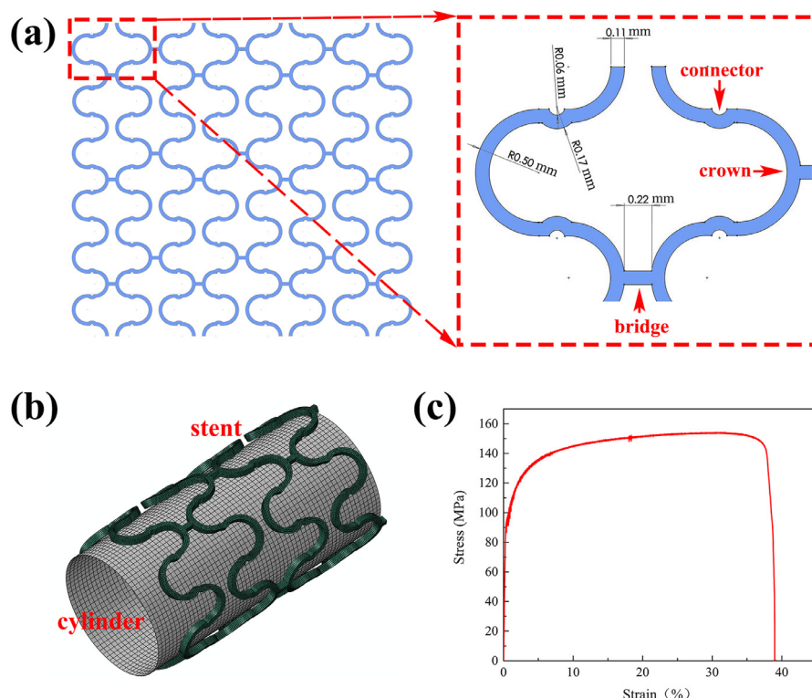
Fig. 1. (a) Schematic pattern design of the Mg-8.5Li stent, with typical regions and dimension parameters shown in the enlarged image, (b) the FEA model composed of a stent and one cylinder, (c) typical tensile curve of the Mg-8.5Li alloy.
