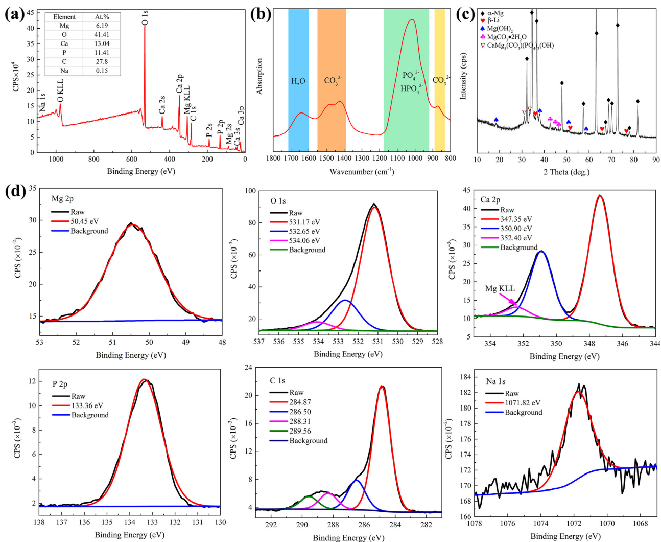
Fig. 6. (a) XPS spectrum, (b) FTIR spectrum, (c) XRD pattern, and (d) high resolution narrow XPS scanning results of the stent (after 7-day immersion in Hank's solution).
