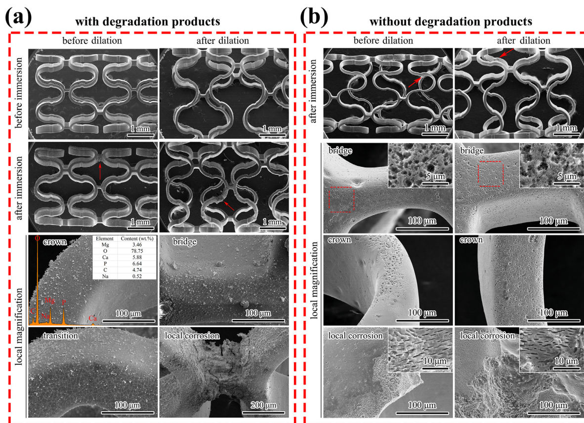
Fig. 4. (a) Microscopic morphologies of the stent (either dilated or not) before and after immersion in Hank's solution for 7 days under SEM, (b) Microscopic morphologies of the degraded stent after removing the degradation products under SEM, with enlargement of typical areas.
