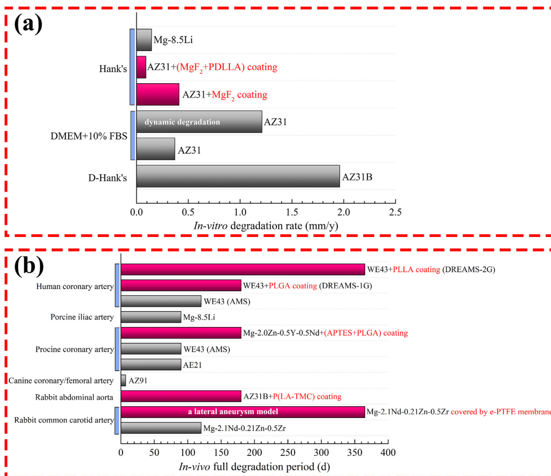
Fig. 9. (a) In-vitro degradation rates of previously reported Mg-based BDSs (with or without coating, the columns of stents with coatings were in magenta) in different mediums, data were from Refs [63–65]. (b) the in-vivo degradation periods of various Mg-based BDSs in different animal models, data were collected from Refs[25–27],[57],[66,67,70,70].
