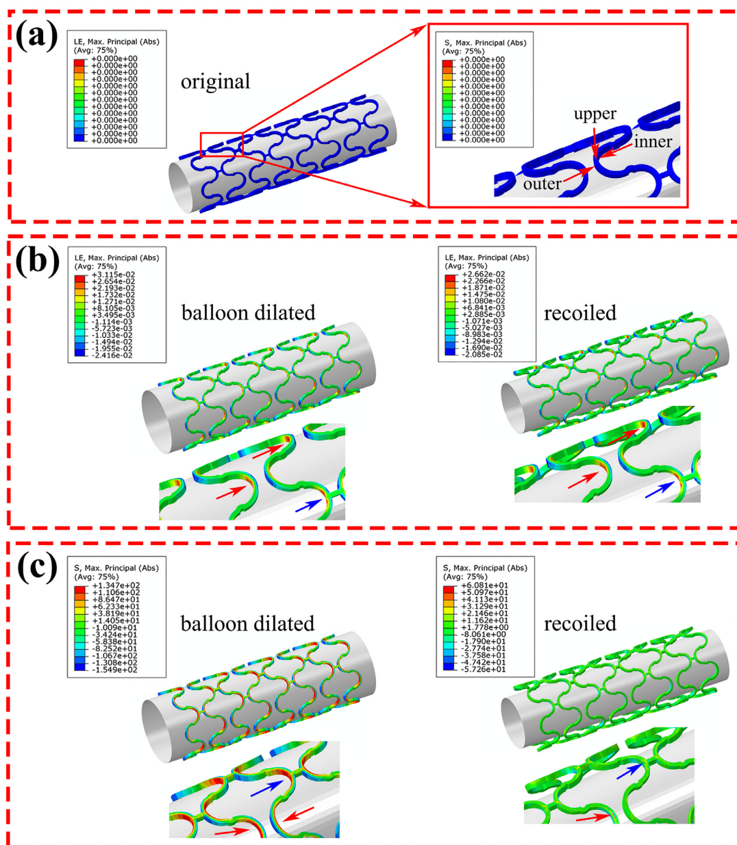
Fig. 2. (a) Typical positions on the stent as indicated by red arrows, (b) the distribution of principal strain on the stent during balloon dilation and natural recoil, red arrows showing the sites with maximum principal strain, blue arrows showing alleviated principal strain at connected neighboring crowns, (c) the distribution of principal stress on the stent during balloon dilation and natural recoil, with red arrows showing the sites with maximum principal stress (tension), blue arrows showing alleviated principal stress at connected neighboring crowns. (For interpretation of the references to colour in this figure legend, the reader is referred to the web version of this article.)
