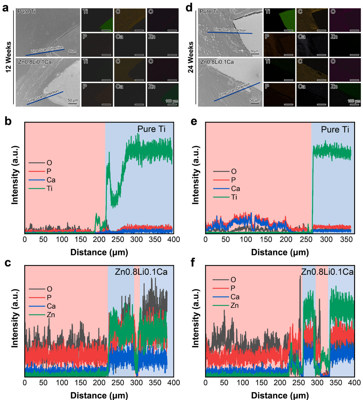
Fig. 7. Elements distribution analysis of hard-tissue slices. (a) EDS mapping of 12 weeks' results; (b) EDS line scan results of pure Ti group at 12 weeks; (c) EDS line scan results of Zn0.8Li0.1Ca alloy group at 12 weeks; (d) EDS mapping of 24 weeks' results; (e) EDS line scan results of pure Ti group at 24 weeks; (f) EDS line scan results of Zn0.8Li0.1Ca alloy group at 24 weeks.
