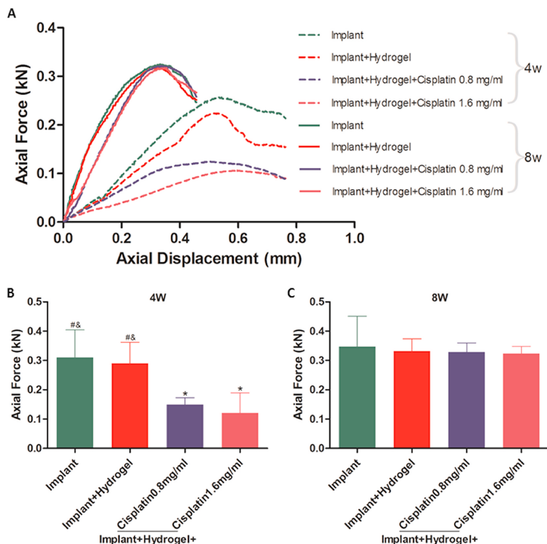
Fig. 7. Fixation strength of the cisplatin/hydrogel-loaded 3D-printed Ti 6 Al 4 V implants in vivo . Push-out tests were performed to obtain the typical displacement curves (A) and the push-out forces at weeks 4 (B) and 8 (C) to evaluate the fixation strengths. Data are represented as mean \pm standard deviation ( n = 5 ). * p < 0.05 , ** p < 0.01 , *** p < 0.001 compared with the implant group; # p < 0.05 , ## p < 0.01 , ### p < 0.001 compared with the implant + hydrogel + cisplatin 0.8 mg/mL group; & p < 0.05 , && p < 0.01 , &&& p < 0.001 compared with the implant + hydrogel + cisplatin 1.6 mg/mL group.
