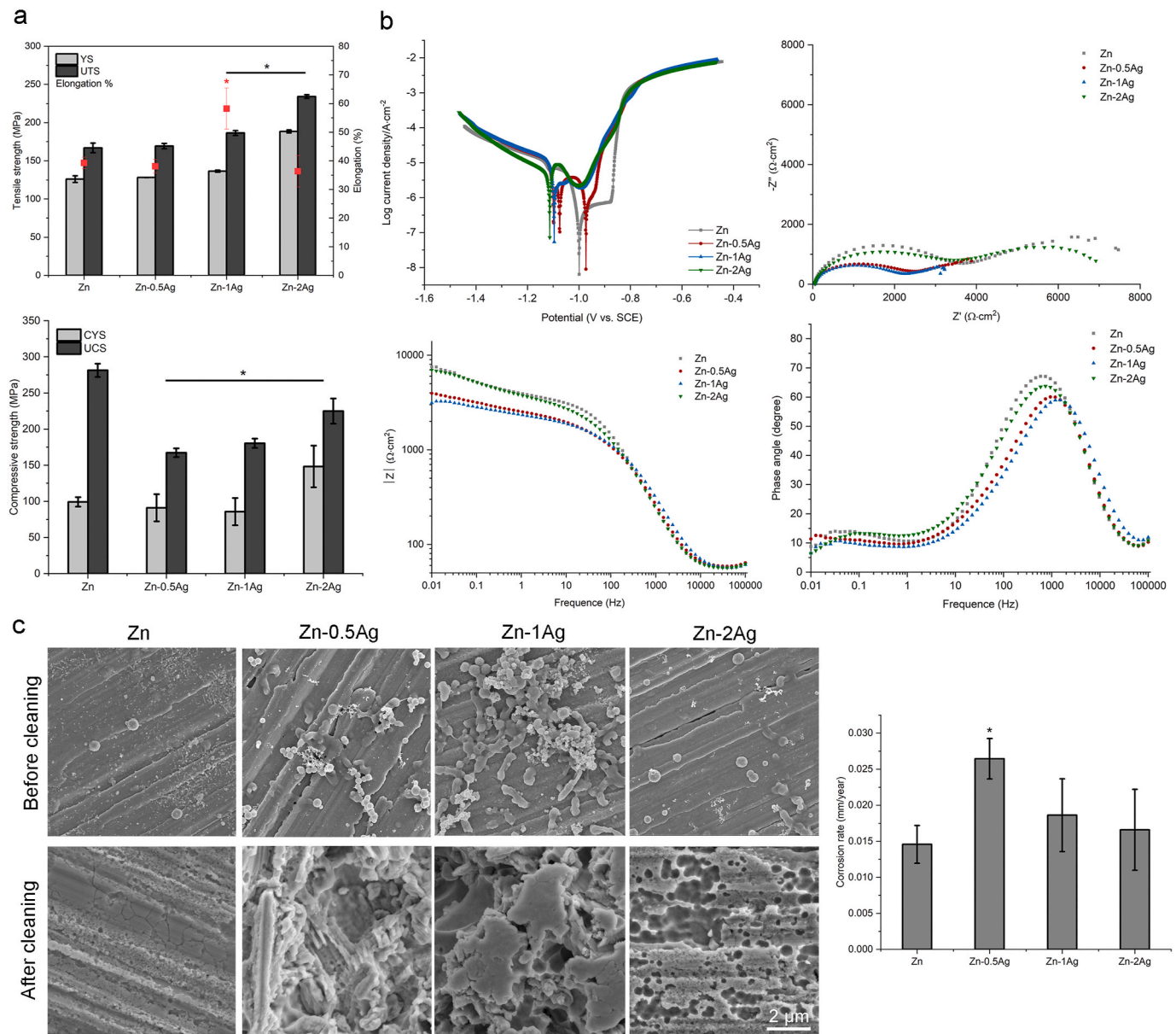
Fig. 1. Mechanical properties and corrosion behavior of Zn–Ag alloys. (a) Mechanical tests: Alloying with 1 and 2 wt% Ag significantly increased the tensile strength of Zn, while maintaining its good ductility; the compressive strength of Zn–Ag alloys decreased compared with that of pure Zn. (b) Electrochemical tests: Electrochemical tests showed that the Zn potential shifted negatively after adding Ag, while its corrosion current density increased greatly. The electrochemical impedance spectra showed that the impedance semicircle radii of Zn–1Ag and Zn–2Ag alloys were smaller than that of pure Zn, indicating a reduced corrosion resistance. (c) Immersion tests: Pure Zn was almost intact after immersion. More precipitates were found on the surface of Zn–Ag alloys. After removal of the corrosion products, pronounced corrosion was observed in Zn–Ag alloys. The intermetallic phases were relatively intact, while the surrounding Zn matrix was severely corroded, indicating a typical galvanic corrosion process. Addition of Ag accelerated the corrosion rate, with Zn–0.5Ag presenting the highest corrosion rate.
