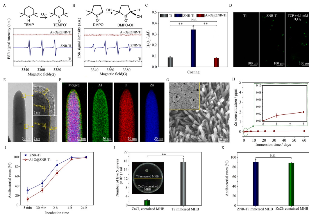
Fig. 7. The ESR spectra of (A) superoxide ( O_2^{\cdot-} ) and (B) hydroxyl radical ( \cdot OH ) in the MHB immersing the bare Ti, ZNR-Ti and Al-O@ZNR-Ti discs as detected using TEMPO and DMPO-OH spin trap agents; (C) the concentrations of H_2O_2 in the MHB immersing the bare Ti, ZNR-Ti and Al-O@ZNR-Ti discs; (D) fluorescent staining images of ROS in S. aureus cultured on bare Ti, ZNR-Ti in MHB and on TCP in 0.1 mM H_2O_2 contained MHB; (E) TEM analyzed microstructures of Al-O@ZNR and (F) the distribution maps of Al, O, and Zn elements detected on the nanorod shown in (E) using TEM-equipped EDX; (G) surface SEM morphology of Al-O@ZNR; (H) Zn^{2+} concentration of the PS solution immersing Al-O@ZNR as a function of immersion time; (I) the reduction percentages of bacteria colony numbers on ZNR-Ti and Al-O@ZNR-Ti surfaces relative to that on the bare Ti after different incubation time (i. e. antibacterial rates); (J) numbers of undiluted bacteria colonies formed by picking up the 24 h-incubated planktonic S. aureus from the Ti immersed MHB and ZnCl_2 contained MHB and re-cultivating on agar for 24 h, along with the inserted optical photograph of these bacteria colonies; (K) the anti-bacterial rates against planktonic S. aureus of the ZnCl_2 contained MHB and ZNR-Ti immersed MHB after incubation for 24 h (* p < 0.05 , ** p < 0.01 ).
