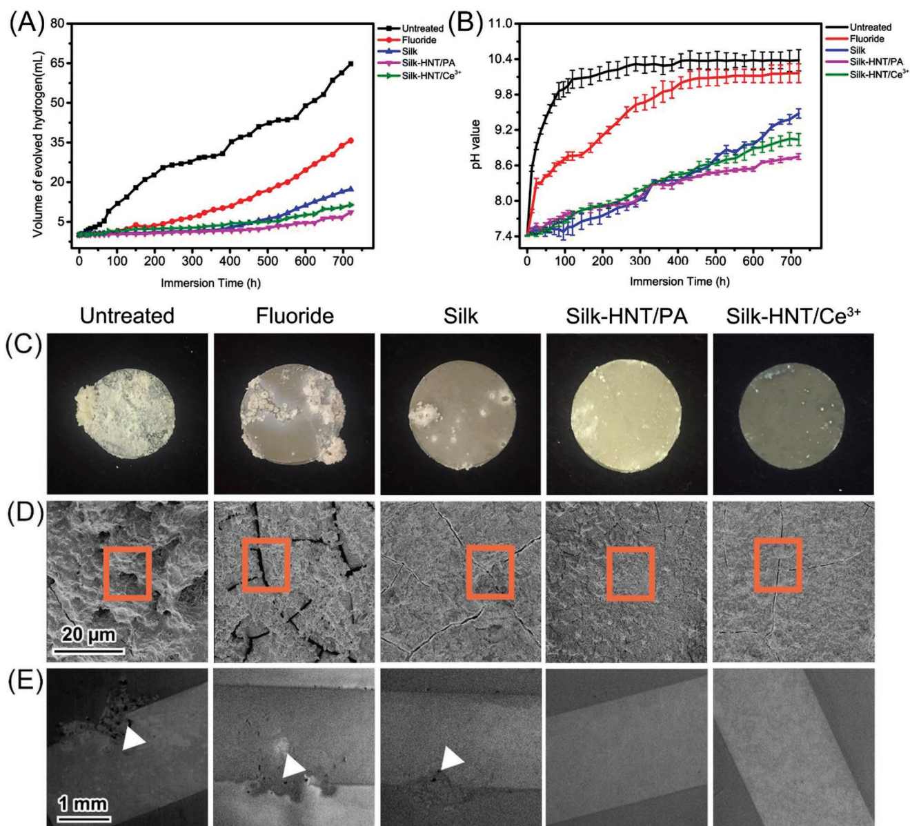
Figure 3. Surface morphology of samples after immersion for 30 days. A) Volume of evolved hydrogen, B) pH value, C) macrograph characteristic, D) SEM images of sample surface, E) SEM images of sample cross-section.
