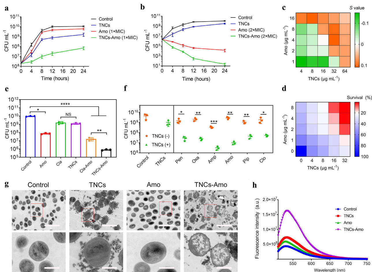
Fig. 2. TNCs potentiate \beta -lactam antibiotic activity in vitro . (a) Growth curves of bacteria under treatment with TNCs, Amo (1 \times MIC), and TNCs-Amo (1 \times MIC) for 24 h. The initial concentration of the bacterial suspension is 2 \times 10^6 CFU mL ^{-1} . (b) Growth curves of bacteria under treatment with TNCs, Amo (2 \times MIC), and TNCs-Amo (2 \times MIC) for 24 h. The initial concentration of the bacterial suspension is 2 \times 10^6 CFU mL ^{-1} . (c) The Bliss Independence model is used to evaluate synergistic interaction between TNCs and Amo. S > 0 indicates a synergistic interaction and S < 0 represents an antagonistic interaction. (d) Survival rate of bacteria treated with Amo at various concentrations combined with TNCs of different concentrations. (e) Comparison of TNCs' ability to re-sensitize antibiotics with Cla's ability to re-sensitize antibiotics. (f) The antibacterial efficacy of Penicillin G potassium salt (Pen), Oxacillin sodium salt (Oxa), Ampicillin sodium salt (Amp), Amoxicillin sodium (Amo), Piperacillin sodium (Pip), and Cloxacillin sodium salt monohydrate (Clo) combined with TNCs after 8 h. (g) Comparison of bacterial transmission electron microscope (TEM) images in the presence of TNCs, Amo and TNCs-Amo. Scale bar (top) = 2 \mu m and scale bar (bottom) = 500 nm. (h) Fluorescence intensity of SYTOX Green of MRSA treated with TNCs, Amo, and TNCs-Amo. Test conditions: \lambda_{ex} = 485 nm, \lambda_{em} = 525 nm. In (a) (b) (e) and (f), the experiments were repeated three times independently with alike results, * P < 0.05, ** P < 0.01, *** P < 0.001, **** P < 0.0001.
