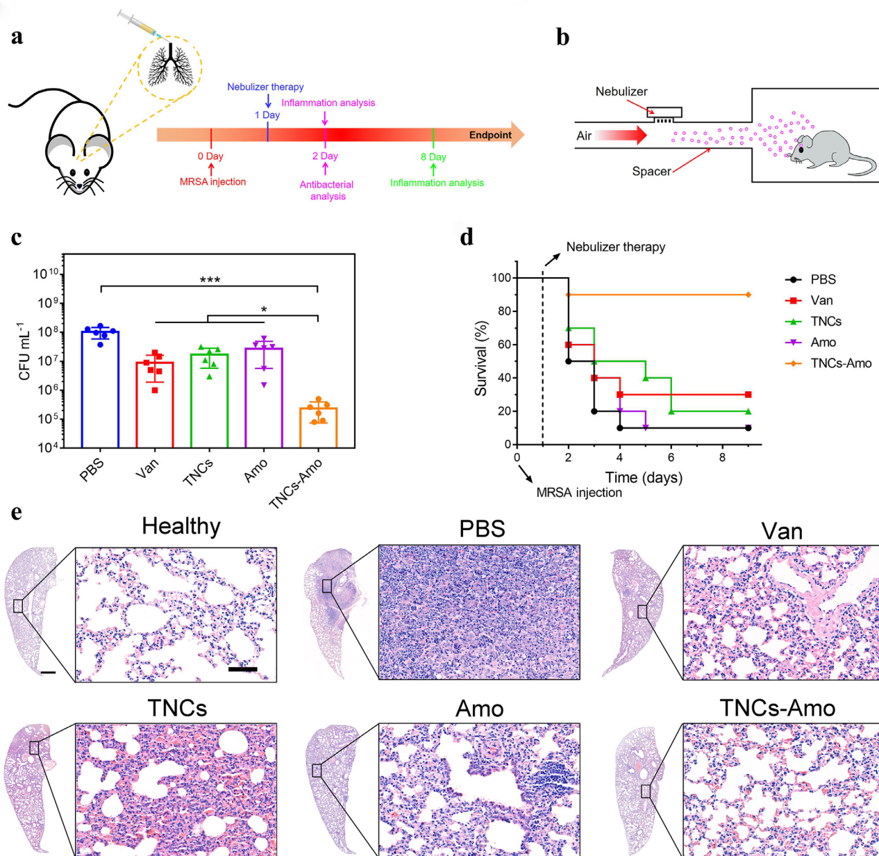
Fig. 5. TNCs enhance antibiotic therapy in vivo . (a) Schematic of the infection and treatment protocol. (b) Pneumonitis treatment diagram for mice. (c) CFU of MRSA in infected lungs after treatment with PBS (control), Van, TNCs, Amo and TNCs-Amo. (d) Survival rate ( n = 10 ) of mice inoculated intratracheally with 5 \times 10^8 CFU of MRSA with the following therapeutics: PBS, Van, TNCs, Amo, and TNCs-Amo. (e) H&E staining images of lungs in mice on day 8. Scale bar (left), 500 \mu\text{m} . Scale bar (right), 50 \mu\text{m} . In c, n = 5 biologically independent experiments. * P < 0.05 , *** P < 0.001 .
